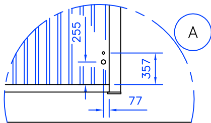
FIXED END ELEVATION
